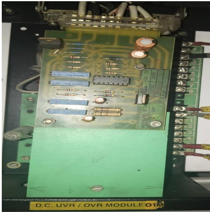
DC U/O voltage PCB with component Material Code: 2000005218
