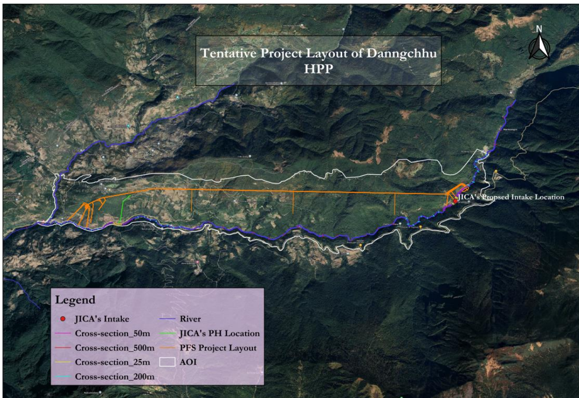
Figure 1 : Tentative Project Layout
