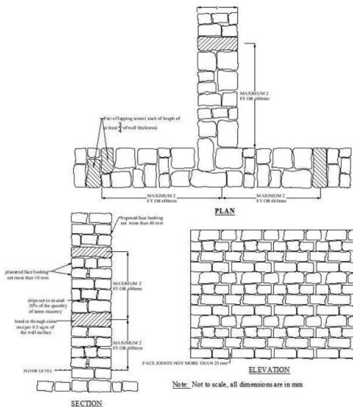
Figure 5.10.1 Random Rubble Masonry
