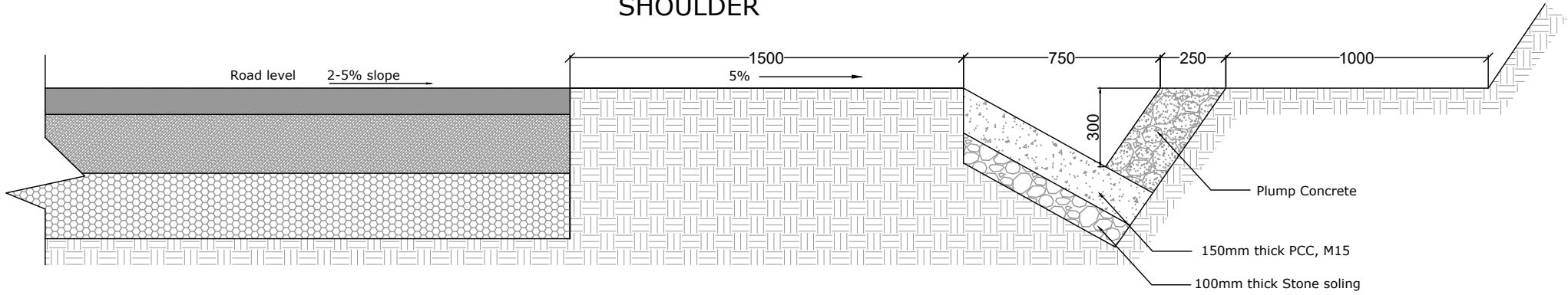
CROSS SECTION DETAILS OF DRAIN
