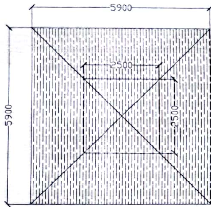
BOTTOM ROOF
