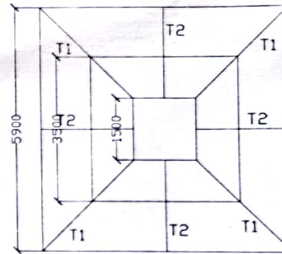
BOTTOM TRUSS LAYOUT
