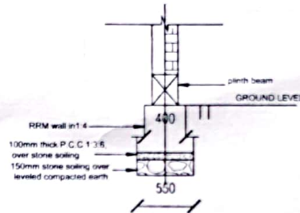
EXTERNAL WALL (250mm) FOUNDATION
