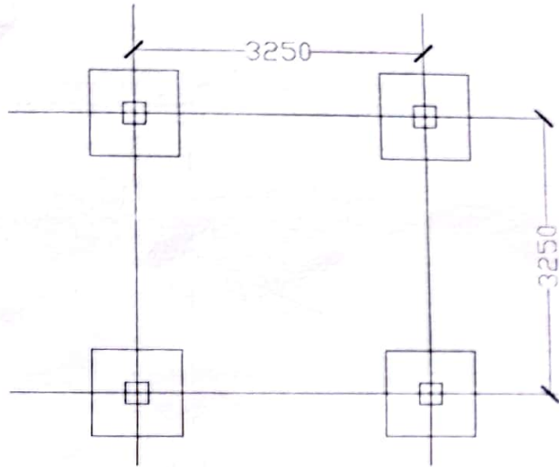
FOUNDATION LAYOUT PLAN
