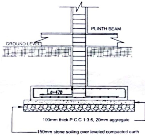
SECTIONAL ELEVATION FOR FOOTING
