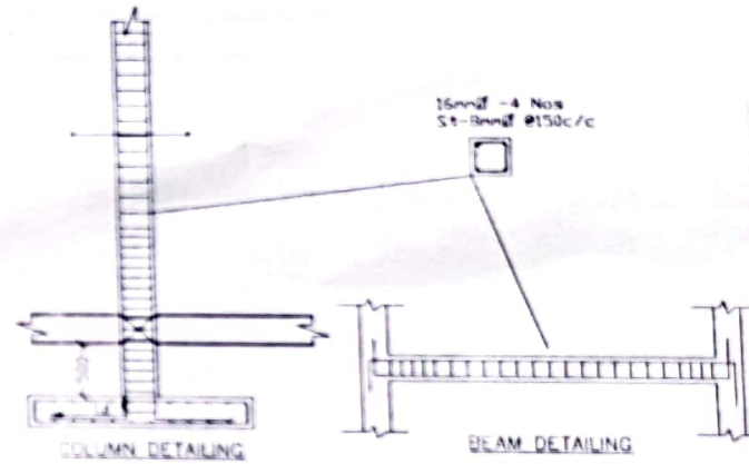
SCHEDULE FOR COLUMN
